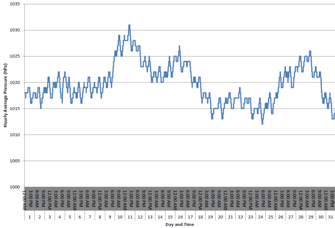
Hourly Average Pressure (hPa) for January 2025
