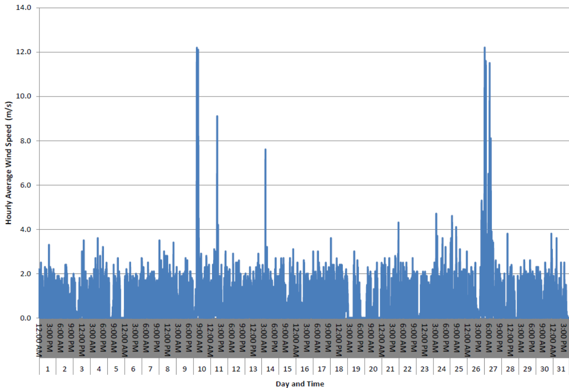
Hourly Average Wind Speed (m/s) for January 2025
